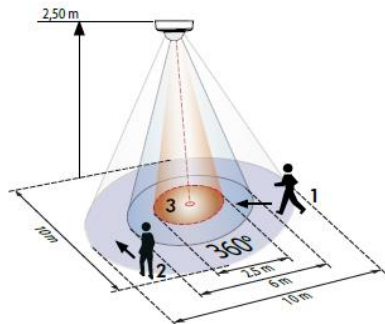
LUXOMAT®PD2-M-2C
