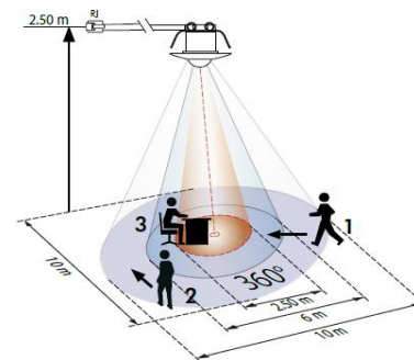
LUXOMAT®PD9-1C-FT
